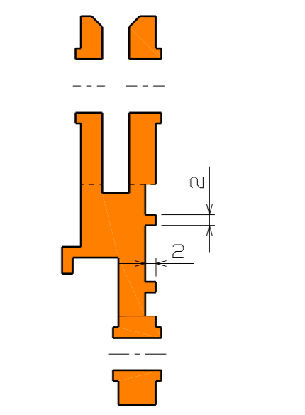
Section Cut A-A
